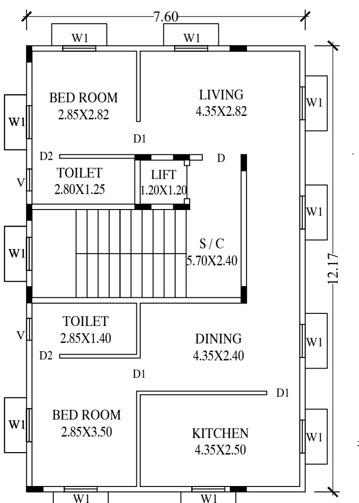
PROPOSED TYPICAL FIRST & SECOND FLOOR PLAN
